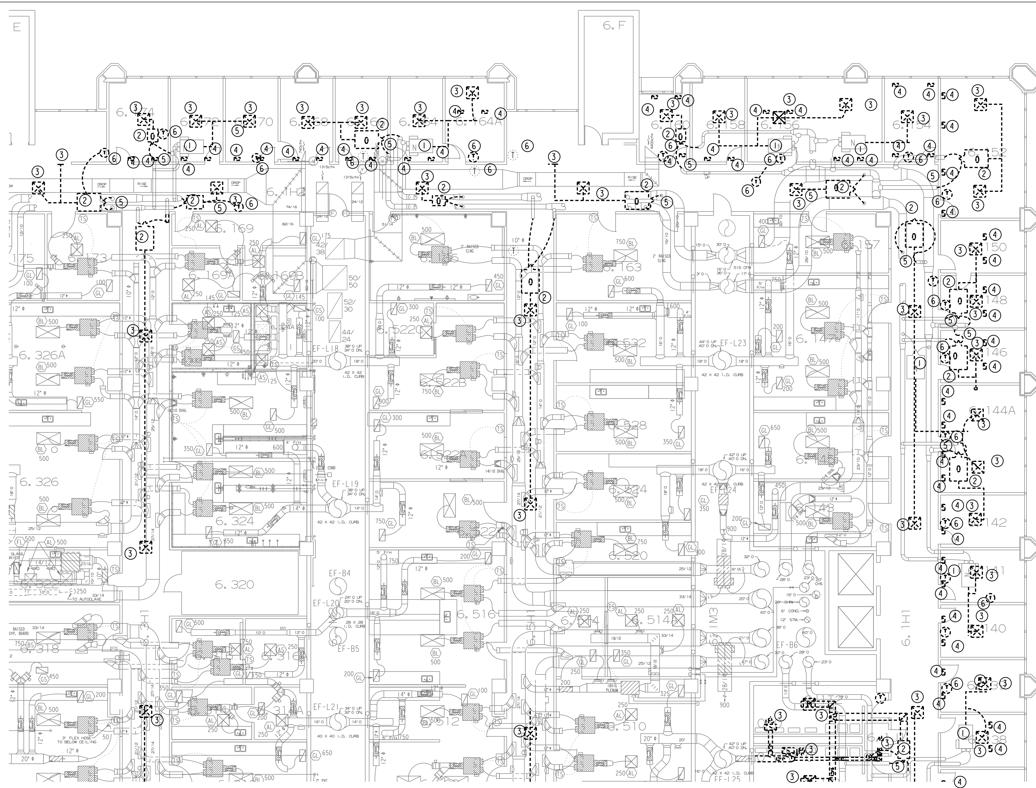
1 MECHANICAL DEMO AREA C PLAN SCALE: 1/8" = 1'-0"
