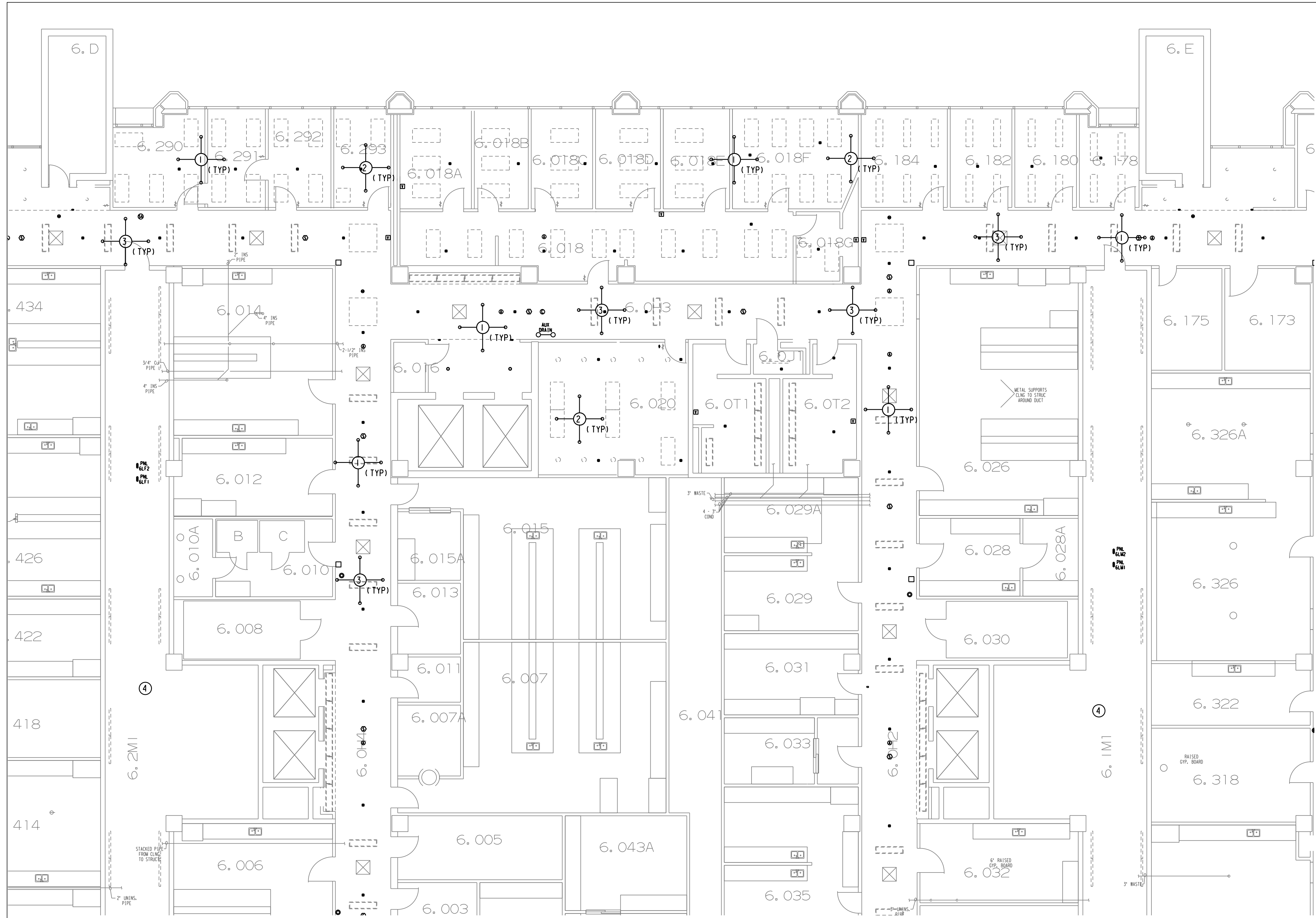
1 ARCH/LIGHTING DEMO AREA B PLAN SCALE: 1/8" = 1'-0"
