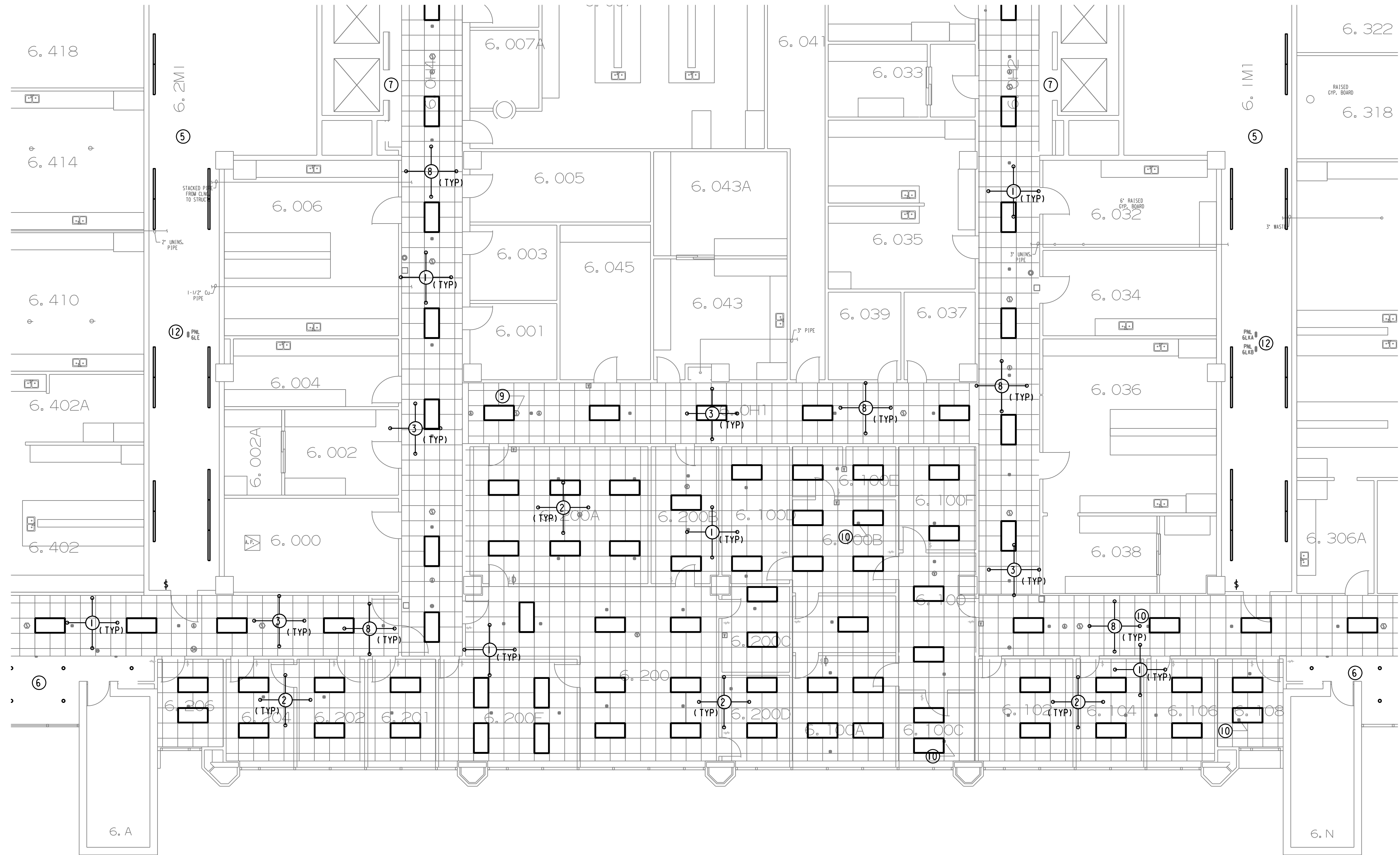
1 ARCH/LIGHTING RENO AREA E PLAN SCALE: 1/8" = 1' - 0"
